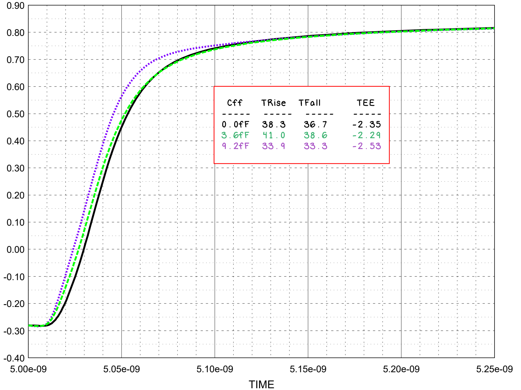
Rise Time Sim - 0, 3.6fF, 9.2fF
